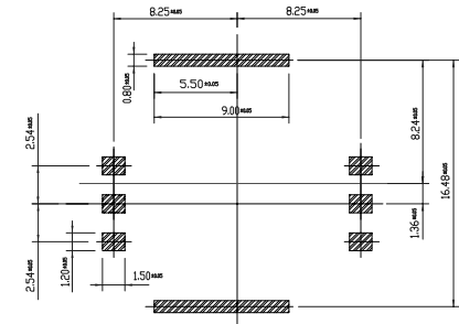
PCB PATTERN
