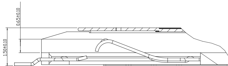
DETAIL B SCALE 16:1
