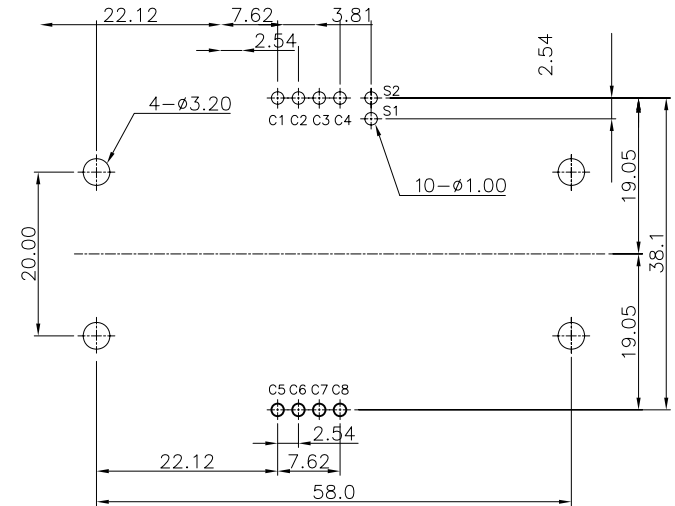
PCB HOLE PATTERN
