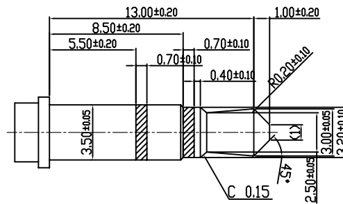
3.5mm 3 POLE PLUG DWG
