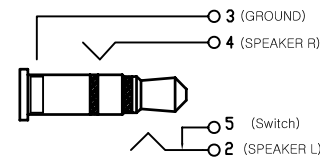
CIRCUIT
