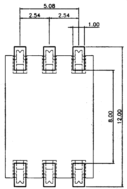
PCB SMD PATTERN
