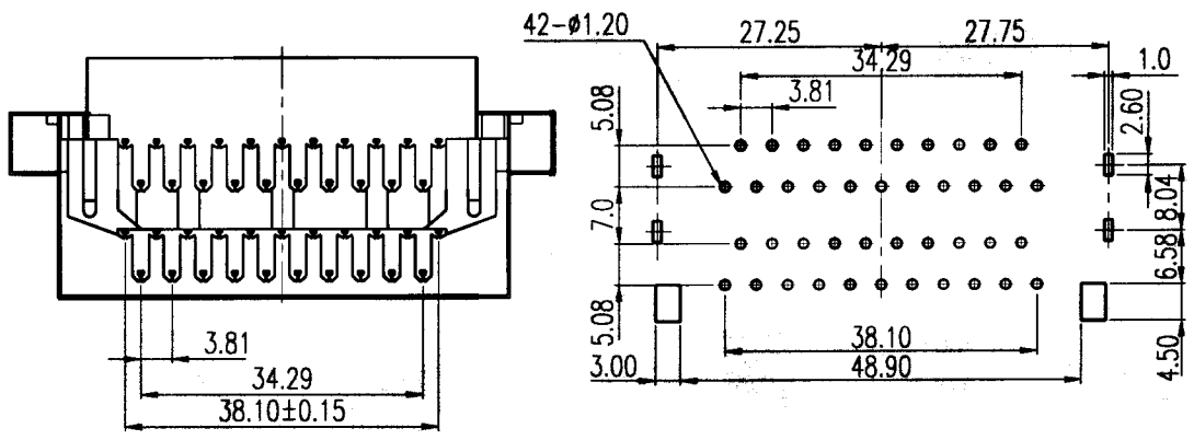
PCB HOLE PATTERN
