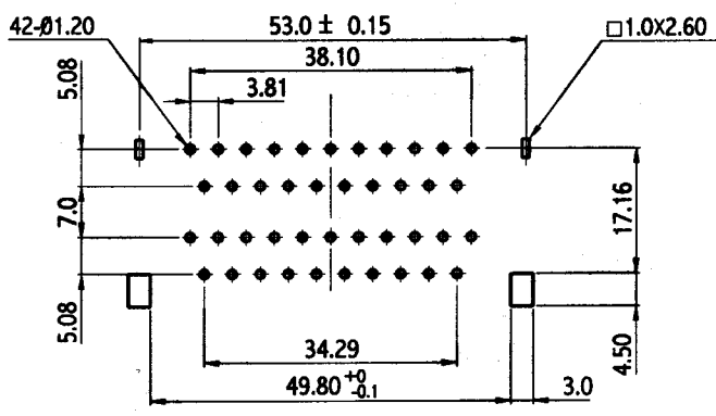
PCB HOLE PATTERN
