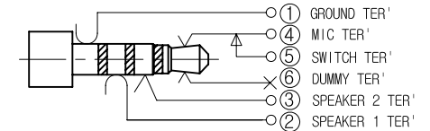
SCHMATIC
