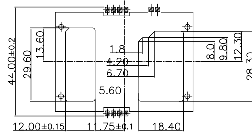
Product Hole Layout
